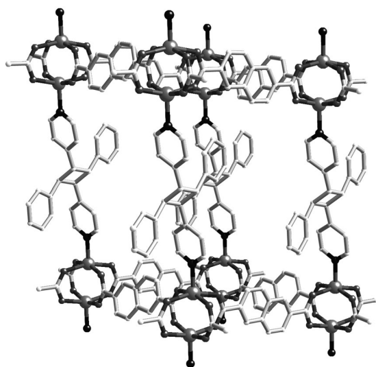
Figure 4. A portion of the pcu connectivity in 2 . Only relevant atoms are shown for clarity. Interpenetration is not shown.
